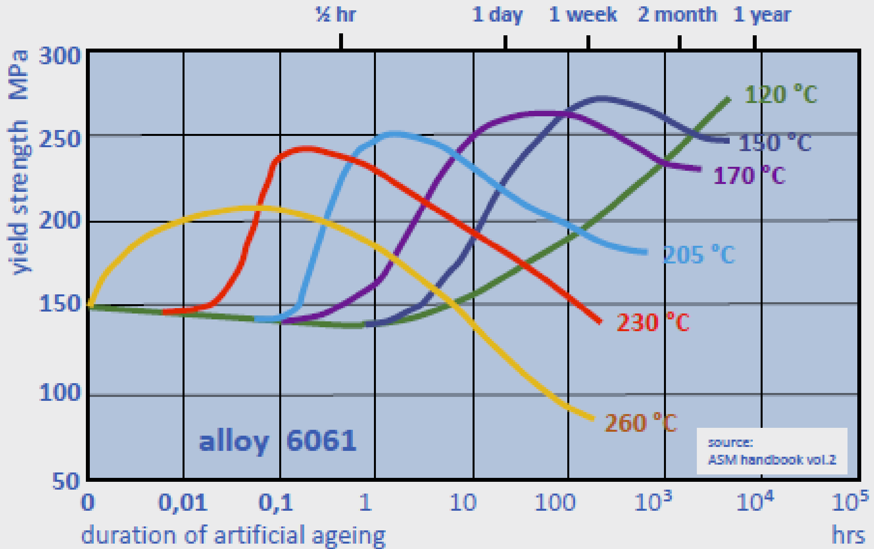
Fig. 9: Effect of different time-temperature artificial ageing parameters
